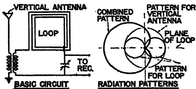
Unilateral direction finder and its radiation pattern.
